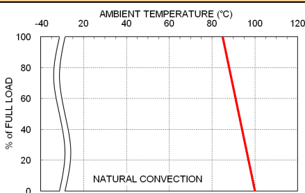
PDL02-24S05 Derating Curve
